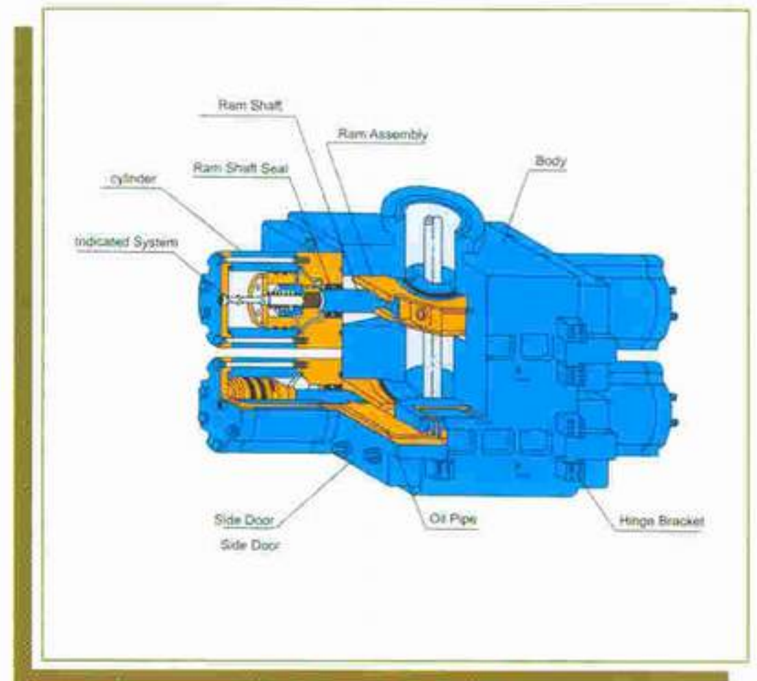
Figure 11- Pipe ram
