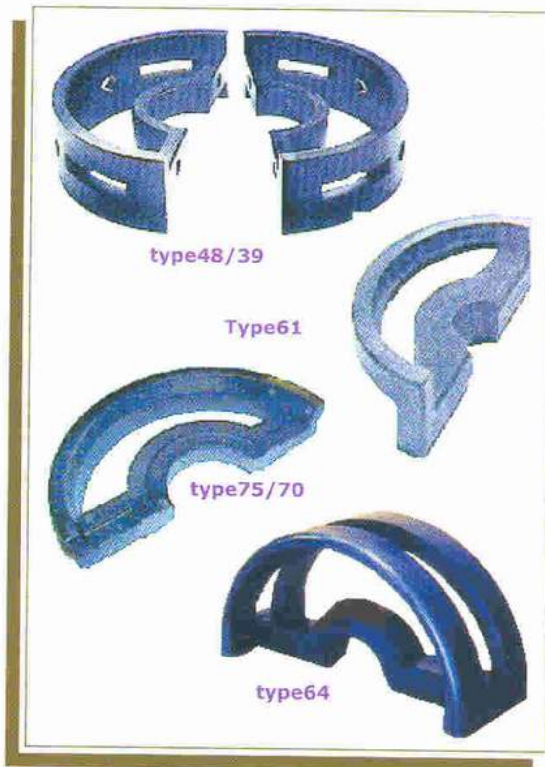
Figure18- Some elastomers for ram-block (Shaffer Co)
