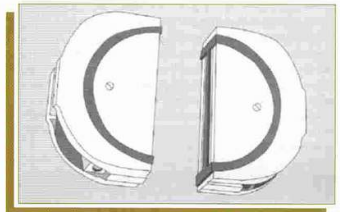
Figure 12- Blind ram
