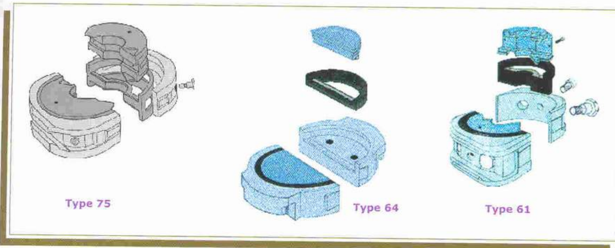
Figure17- Some ram-block assemblies (Shaffer Co)
