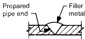
Butt weld For metal thickness of 3/4-inch or less
