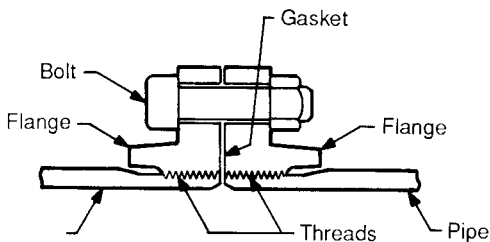
FIGURE C13.9 Flanged joint.
