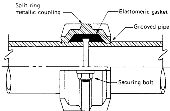
FIGURE C13.8 Grooved joint.
