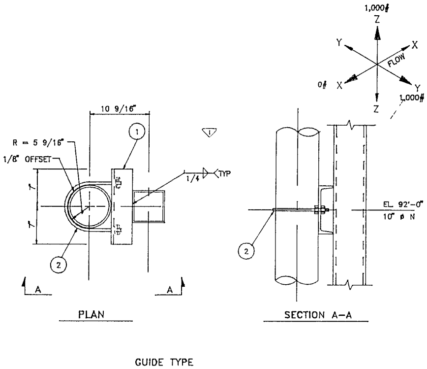
FIGURE C14.19 Sliding pipe support.
