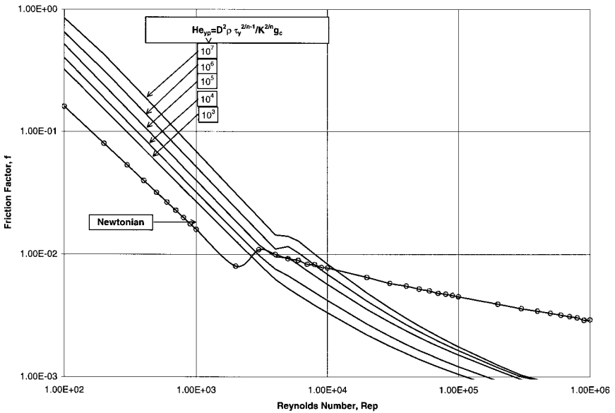
FIGURE C11.9c Friction factor f as a function of Reynolds number for yield pseudoplastic slurries for n = 0.3 , He = [D^3 \rho \tau_y (t/K)^{2/n-2}] / (K^2 g_c) , Re = 8 \rho D^2 V^{2-n} [n/(2 + 6n)]^n / (Kg_c) , where D = pipe ID (ft), V = velocity (ft/s), \rho = density (lb/ft 3 ), K = consistency (lb \cdot s n /ft 2 ), \tau_y = yield stress (lb/ft 2 ), g_c = 32.2 (lb \cdot s/(lb \cdot ft 2 )).
