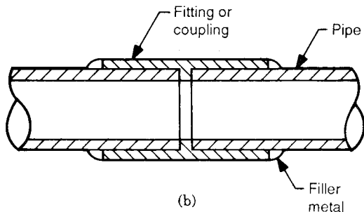
FIGURE C13.10 (a) Butt-weld joint. (b) Socket weld joint.
