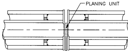
FIGURE B13.85f Plane the ends of the pipes to be sure that they are parallel and to expose a clean surface for welding.
