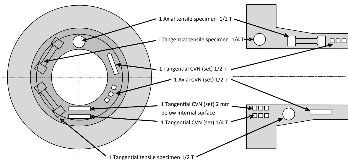
Figure 1 Location of tensile and CVN specimens, component with section thickness ≥ 25 mm
